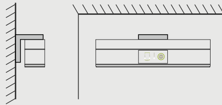
Ceiling mounting with the A-2138
