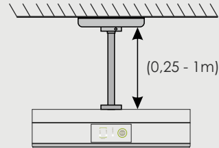
Hanging ceiling mounting up to 1m with the A-2130, A-2031, A-2132
